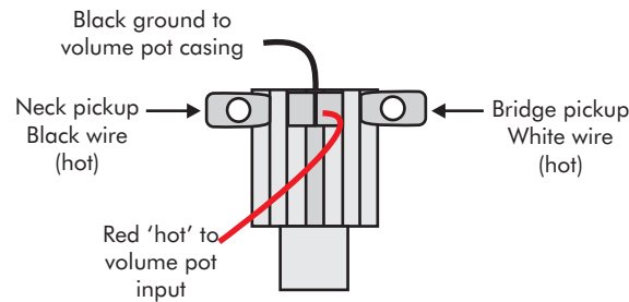
3-way pickup selector switch:
