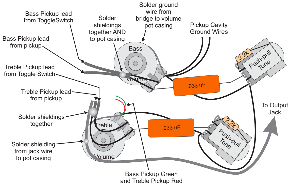
Push-pull tone pot (Bass Pickup):
