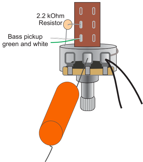
Push-pull tone pot (Bass Pickup):
