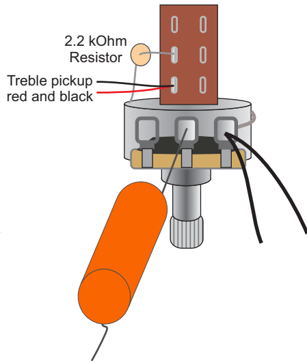
Push-pull tone pot (Treble Pickup):
